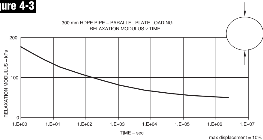
Figure 4-3: Stiffness Relaxation
